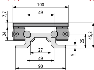
LFS-12-3 equipped with aluminum slide type WS 7
