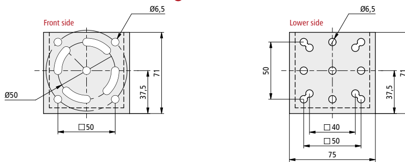
WV 1: L 71 x W 75 x H 71 mm
